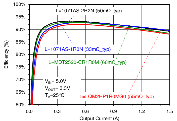
Efficiency vs. Load Current ( V_{IN}=5.0V, V_{OUT}=3.3V )
